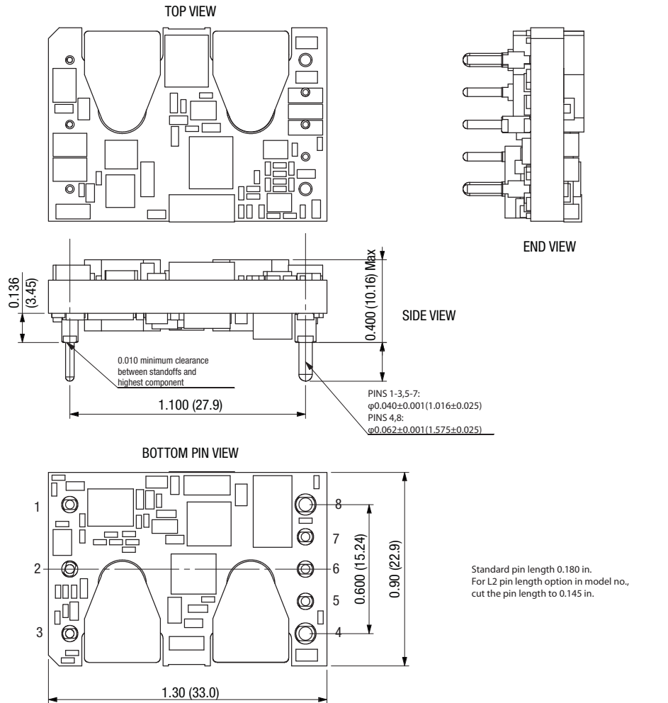
RECOMMENDED FOOTPRINT (VIEW THROUGH CONVERTER)
